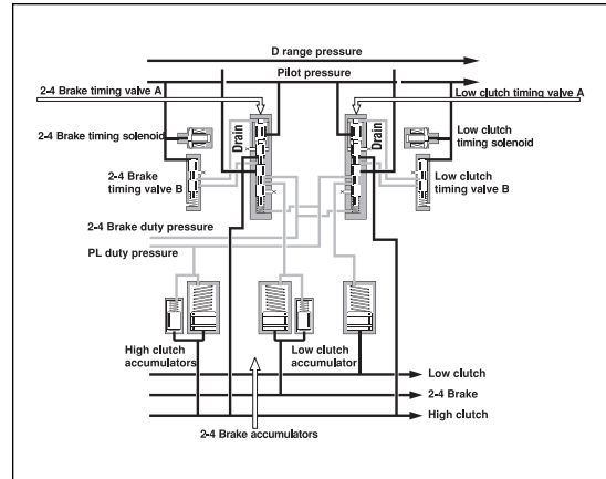
2-4 Brake Timing
